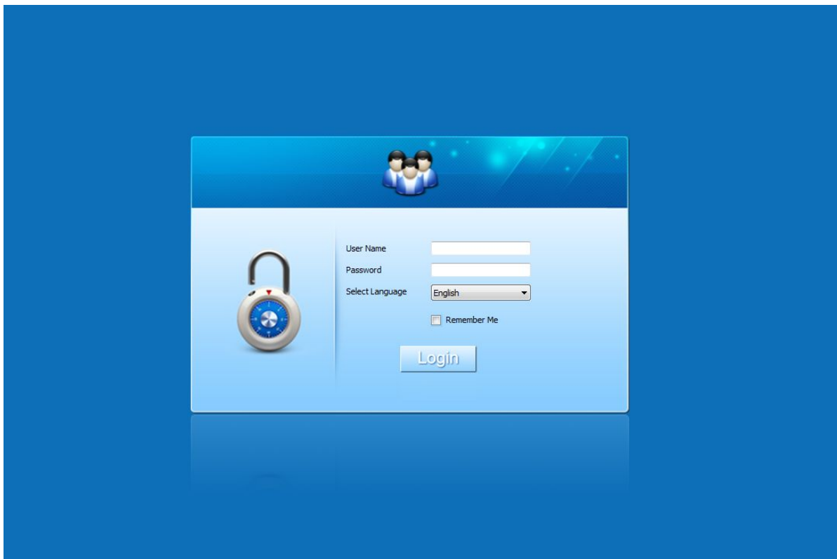
Figure3- 1 Login interface
