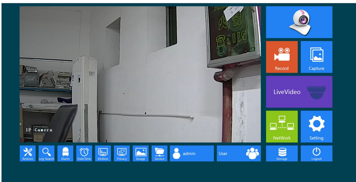
Figure3- 2 Main Interface
